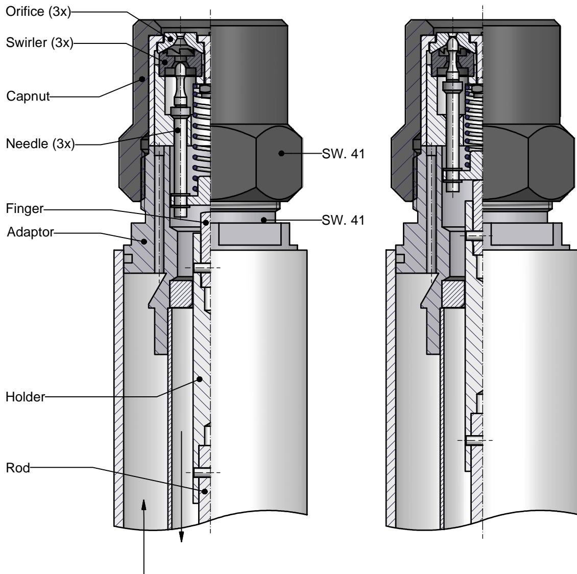
Needle open
