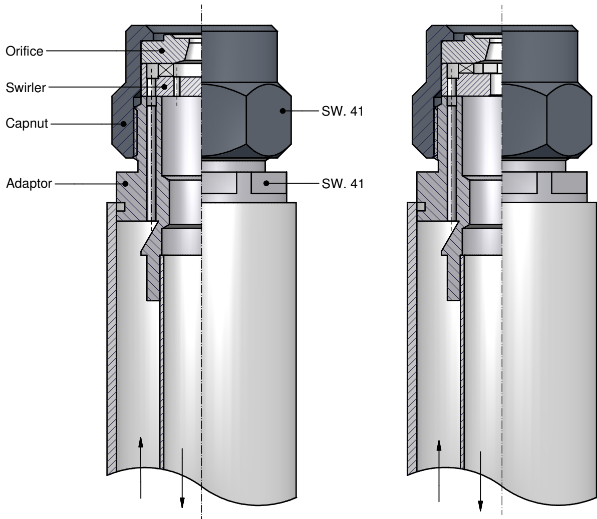
Ringbores
